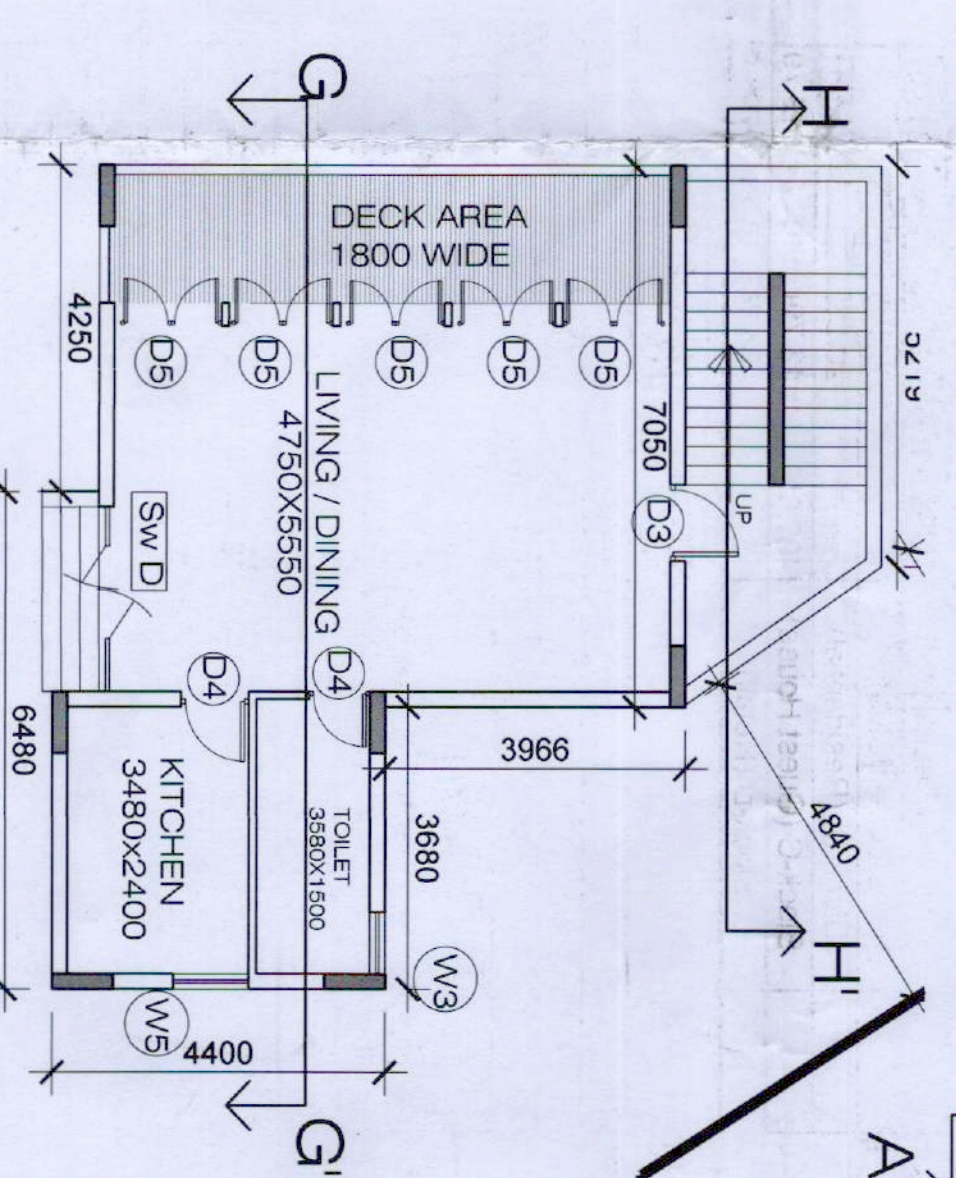
GROUND FLOOR PLAN (BLOCK -C)
